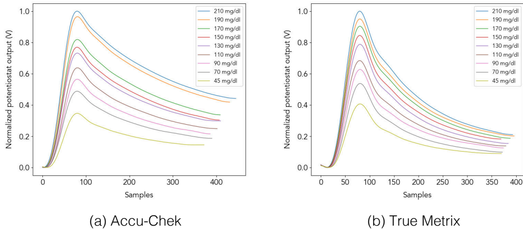
Figure 3.5: One repetition of data collected from a Google Pixel 5 phone during a single session for all glucose solution concentrations utilized in the in vitro testing. Figures (a) and (b) exhibit results from the GlucoScreen prototype with Accu-Chek and True Metrix test strips, respectively. The Y-axis represents amplitude on both graphs; the X-axis represents data samples. The plotted data is shown after pre-processing. Each curve depicts the response of the GlucoScreen prototype to a single solution; the lowest curve depicts the lowest concentration, while successively higher curves represent higher concentrations.
