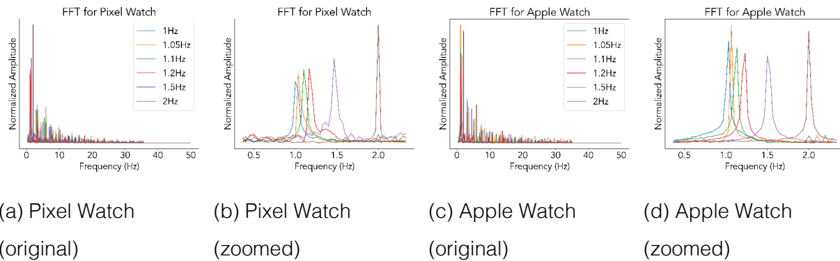
Figure 5.9: Spectrograms from the frequency resolution study for Apple and Pixel Watches (with the right-side images being zoomed-in versions of the left ones), illustrating six frequency responses triggered by a single frequency application on the watch. The plots on the right show that both watches can distinguish frequencies as close as 0.05 Hz.
