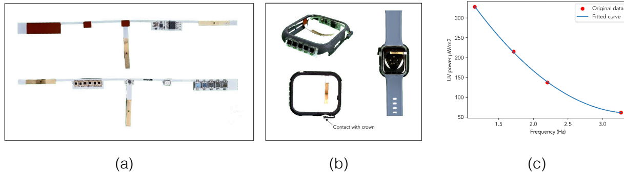
Figure 5.11: (a) The UV light sensor from both front and back is built on a flexible PCB with a design that allows it to be integrated into a 3D printed case designed for the Apple Watch. (b) The case is equipped with the PCB, demonstrating how the case engages in sliding contact with the watch's crown and how the PCB establishes a connection with the watch's ground. (c) A graph depicting the correlation between the sensor's prediction of UV light intensity and the actual measured values.
