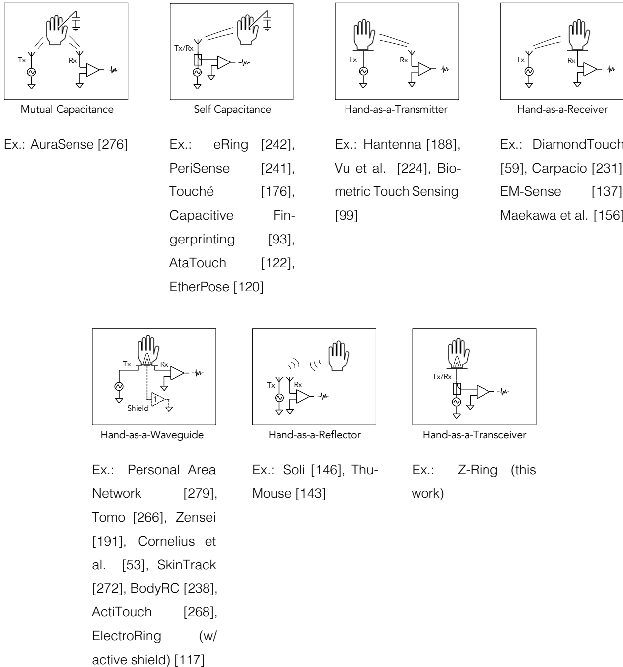
Figure 6.2: Various electric field sensing topologies categorized by transmit and receive antenna coupling configuration (see [280, 82]). Z-Ring’s unique topology combines and extends elements of existing topologies. Note: Body capacitance to ground is present in all systems but is omitted here, where it is parasitic rather than utilized for sensing.
